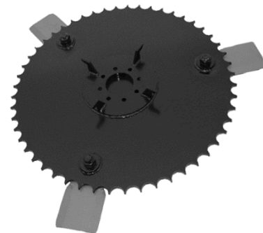
Blade carrier for 48" cutter (wire guard for gear box seal protection)
