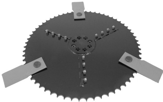
Blade Carrier Shown with optional Bolt-on Mulching Teeth
