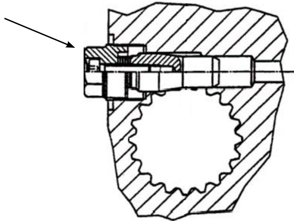
Clamping cone
